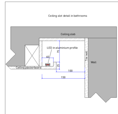
Slot detail in the ceiling washing down the wall.
