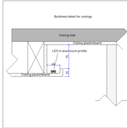
Bulkhead lighting.
