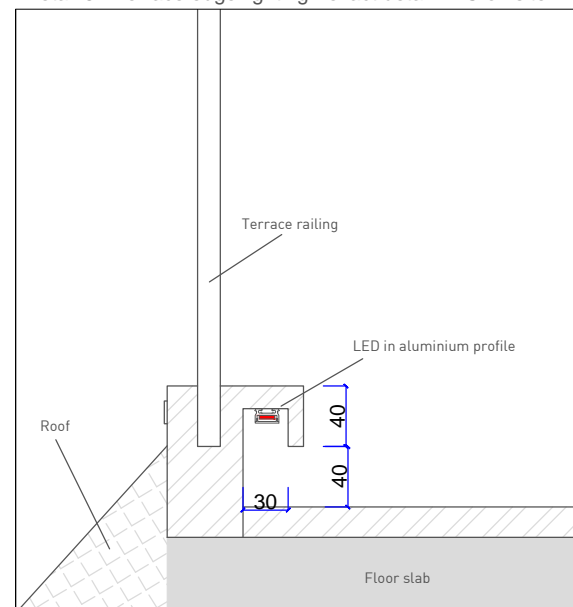
Detail 6 - Terrace edge lighting - exact detail TBC on site
