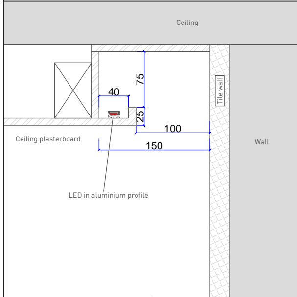
Detail 3 - Shower ceiling slot detail
