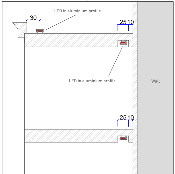
Detail 1 - Kitchen tall unit
