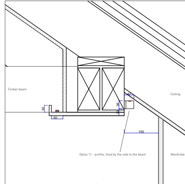
Detail 5 - 1:10 scale - Wardrobe front lighting & ceiling uplight
