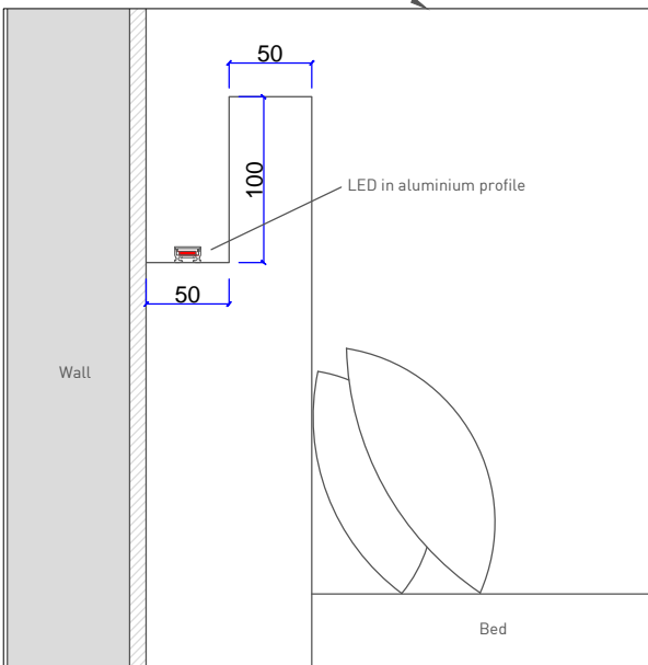
Detail 4 - Headboard lighting
